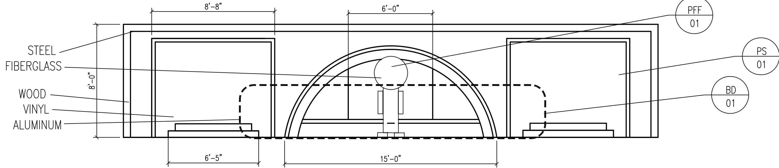
1 Front Full View 1/4 inch = 1'-0"
