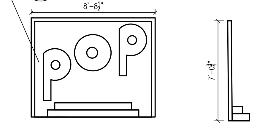
4 Photo Spot 1/4 inch = 1'-0"
