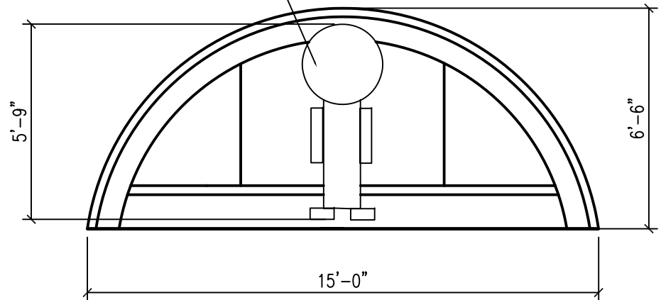
3 Front Section View 1/4 inch = 1'-0"
